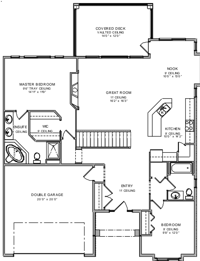
Erickson MAIN FLOOR 1502 SQ FT
