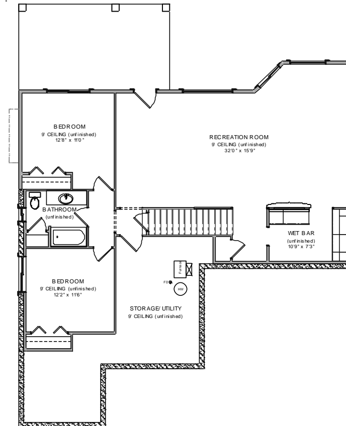
Galena LOWER FLOOR 1599 SQ FT OPT FINISH 1217 SQ FT
