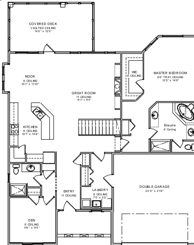
Galena MAIN FLOOR 1635 SQ FT
